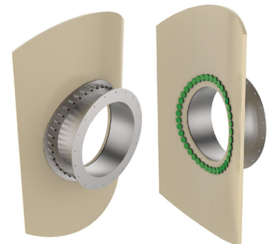
6"-24" SS and FRP Radiused Fittings
